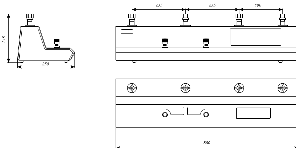
PSKA: control panel
